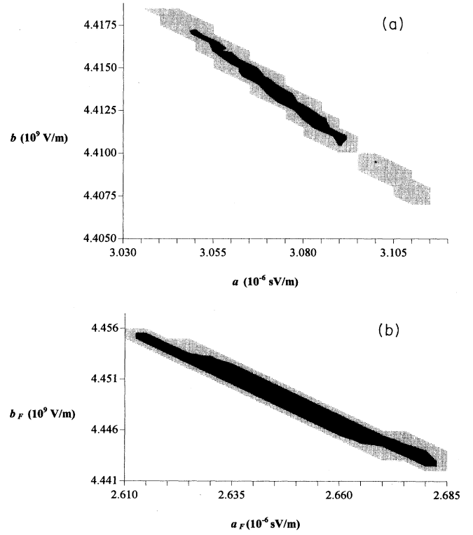
FIG. 2. The \chi^2 contour plots for the fits of the two parametrizations of the lifetime formula (a) \tau = (a/F)\exp(b/F) and (b) \tau = [a_F/(1 - \eta F)]\exp(b_F/F) for a beam energy of 797 MeV. The darker interior region is the 1\sigma confidence interval, and the outer gray region is the 2\sigma confidence interval. The jagged nature of the confidence intervals reflects the graininess of the calculations.
