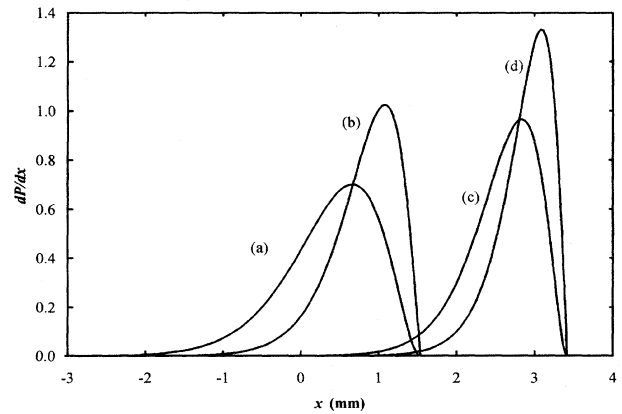
FIG. 5. Predictions for probability density distribution functions using the present experimental apparatus for the M=0 component of the 2p^2\,^3P^e and the M=\pm 1 components of the 2s3p\,^3P^o(2) states of H^- for Gypsy magnet peak field settings of 0.6 and 1.3 T. The lifetime values are based on fitting the calculational results of Ho (Ref. [12]) to the function \tau = (a/F)\exp(b/F) . Curves (a) through (d) are for the following states and field values: (a) 2p^2\,^3P^e at 0.6 T, (b) 2s3p\,^3P^o(2) at 0.6 T, (c) 2p^2\,^3P^e at 1.3 T, and (d) 2s3p\,^3P^o(2) at 1.3 T. The x locations of the peaks of the curves are at 0.65, 1.40, 2.83, and 3.02 mm, with FWHM values of 1.4, 1.07, 0.70, and 0.86 mm, respectively.
